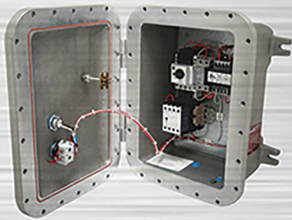
Full Voltage Motor Control
